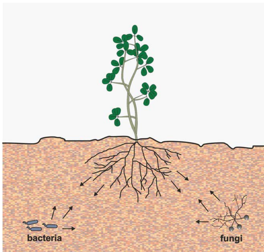
Molecular dialogues in plant-microbe symbioses.
